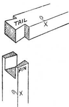
Figure 3: Dovetail joint.
